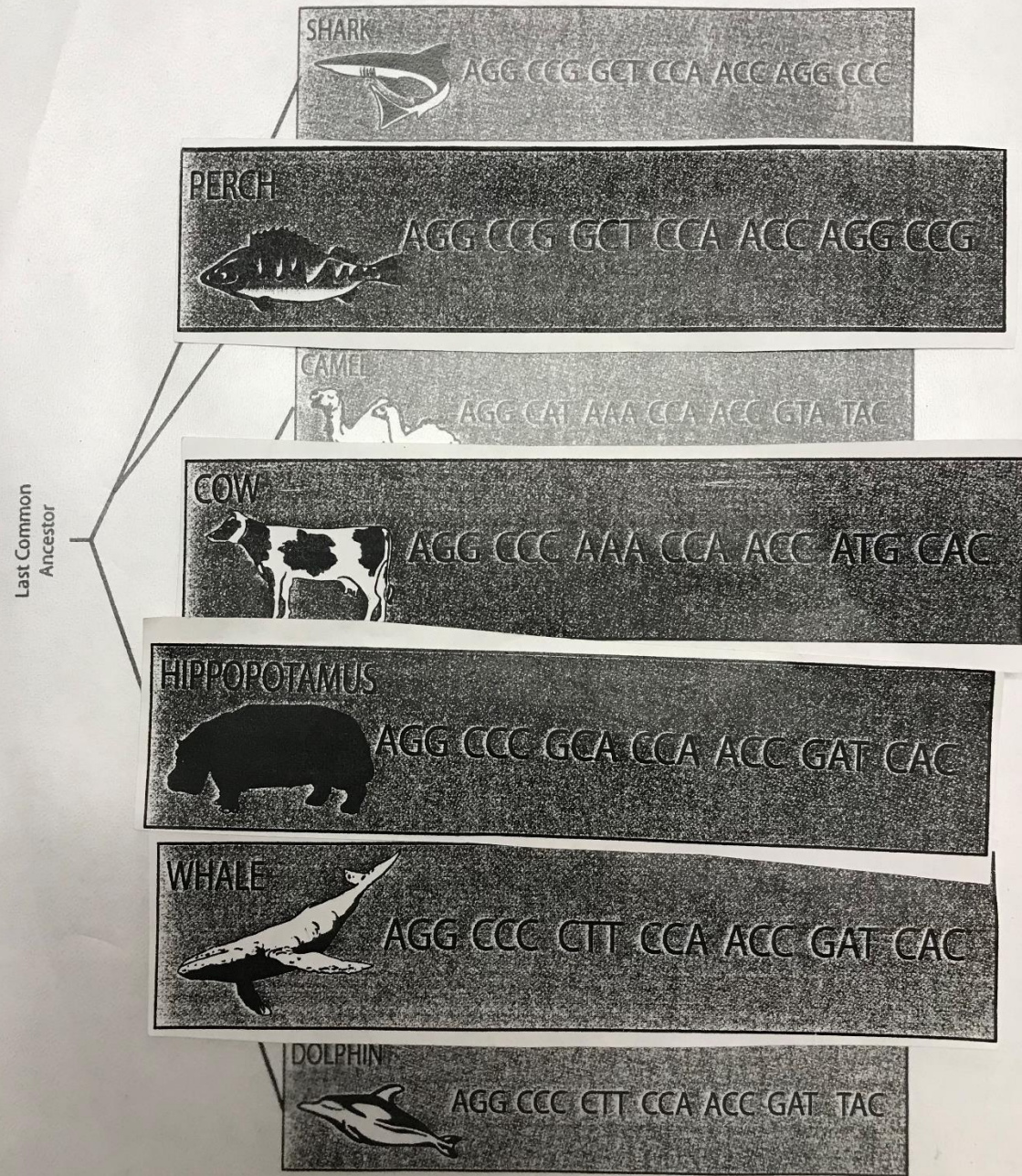
DNA Sequence Cladogram
